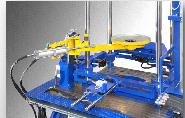
gefederter Ablageteller
